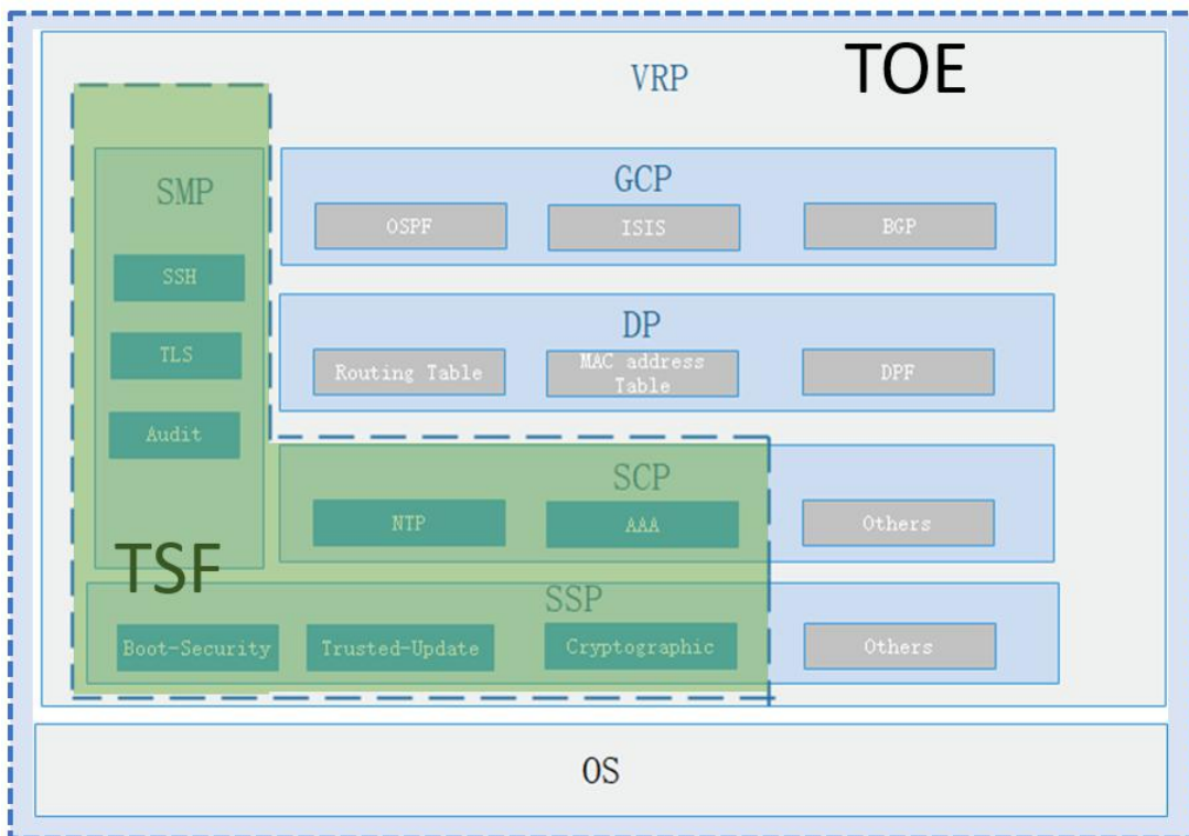
Figure 2 Architecture and boundaries of the Target of Evaluation
